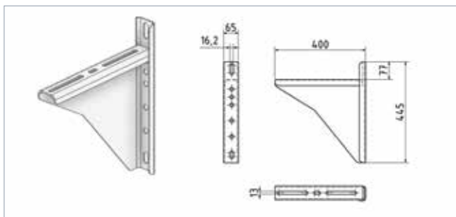
DIMENSIONS OF BRACKET ATTACHMENT 7.0
